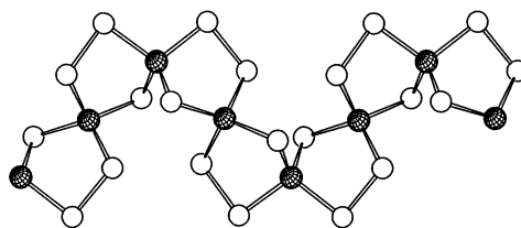
(c) {}^1_\infty[\text{In}_2\text{Te}_6]^{2-} in 8 period = 11.55 Å
