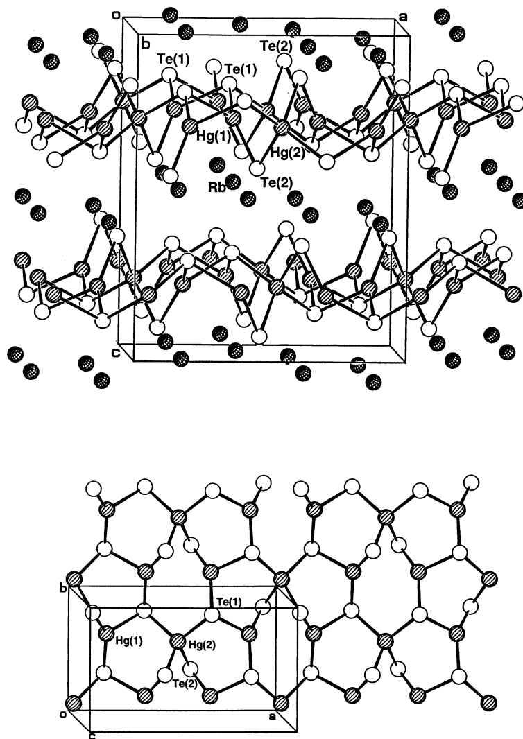
Fig. 15. Crystal structure of 23 showing a perspective view along the b axis (top) and a single layer of {}^2_{\infty}[(\text{Hg}_3\text{Te}_4)^{2-}] (bottom).
