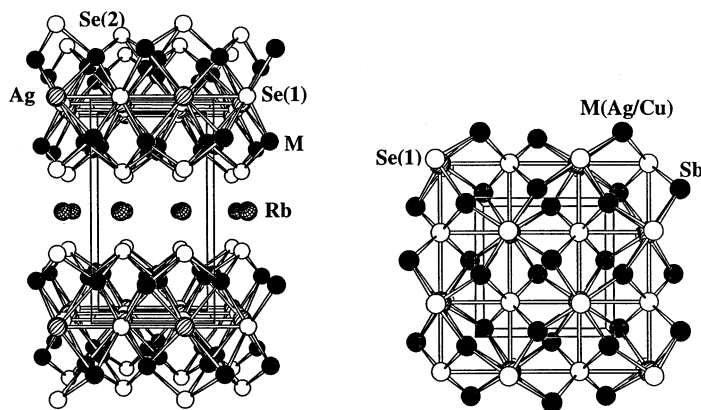
Fig. 13. Left: a perspective view of 21 showing the \frac{2}{\infty}[(\text{Cu}_{1.2}\text{Ag}_{3.8}\text{Se}_3)^-] 2D layers and \text{Rb}^+ cations located between the layers. Right: a single layer of \frac{2}{\infty}[(\text{Cu}_{1.2}\text{Ag}_{3.8}\text{Se}_3)^-] .
